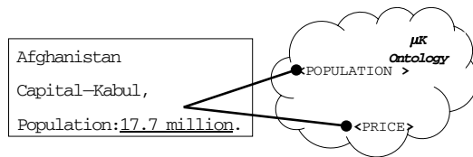
Fig. 4. Matching concepts via data frames
