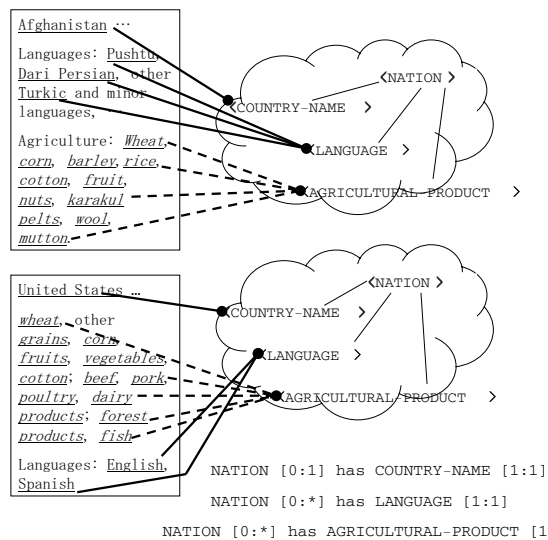
Fig. 7. Generating participation constraints
