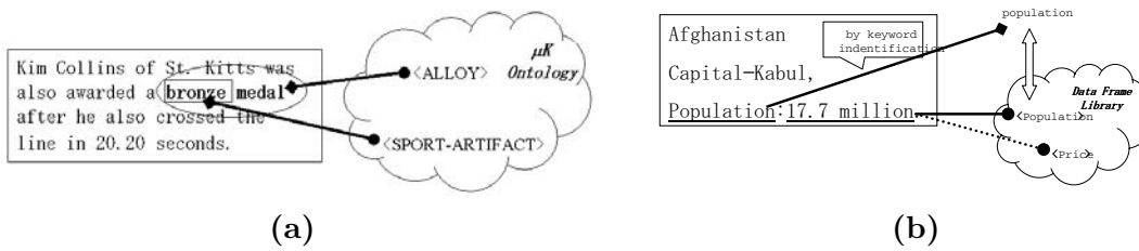
Fig. 6. Resolution via: favor longer over shorter (a), and context decides meaning (b)
