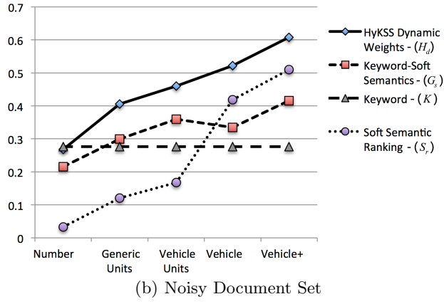
Fig. 8. Representative MAP Scores
