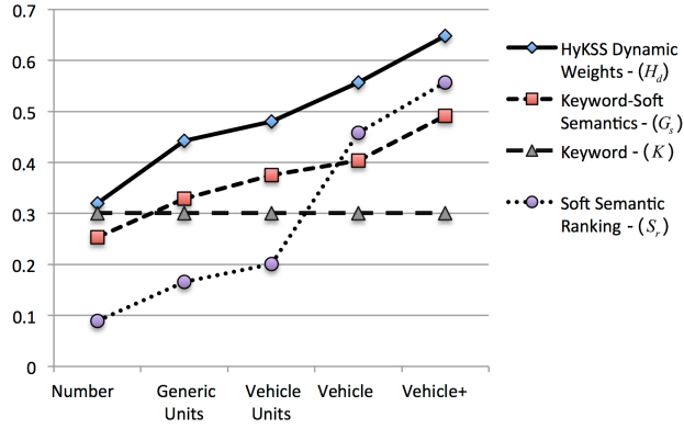
Fig. 9. Representative MAP Scores Averaged over Document Set
