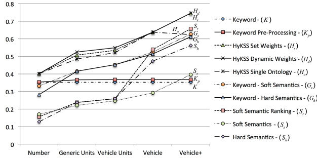
Fig. 7. MAP Scores for Training Query Set and Clean Document Set
